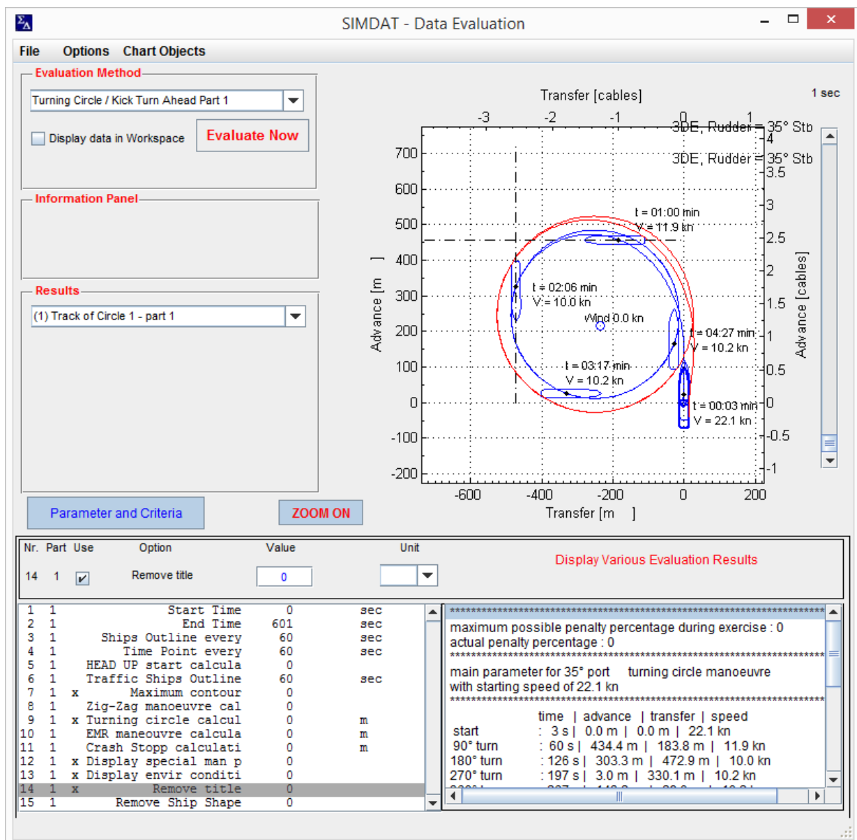
Fig. 5 - SIMDAT data evaluation of a turning circle from simulation data
