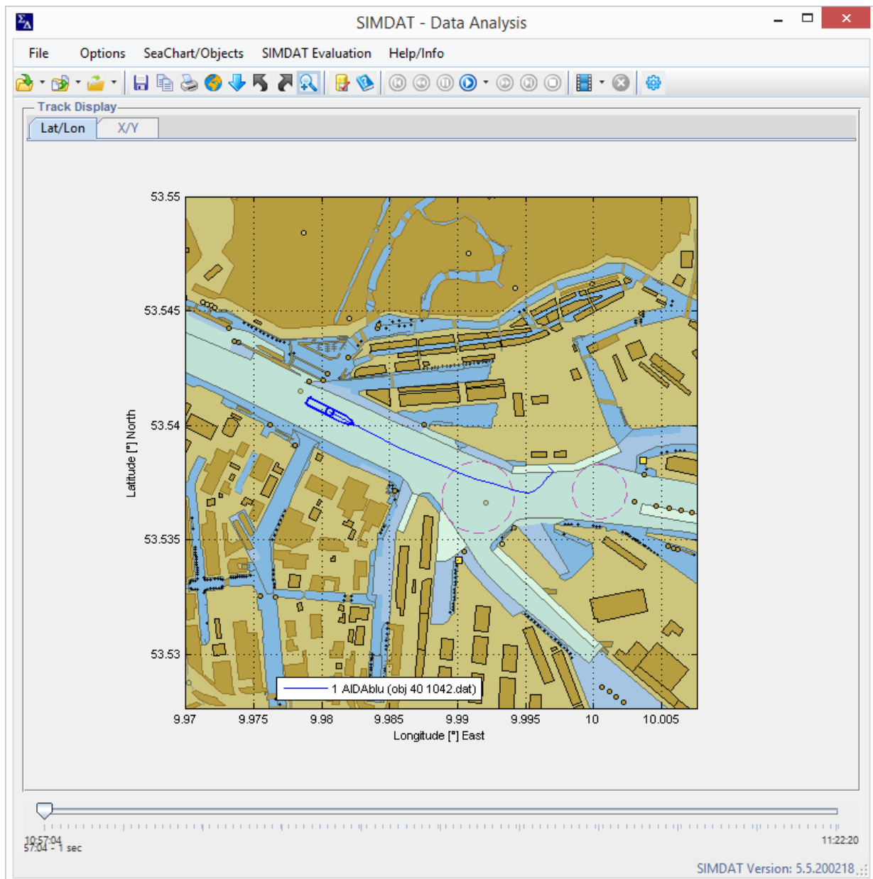
Fig. 2 - SIMDAT main window with maximized track display together with Electronic chart data
